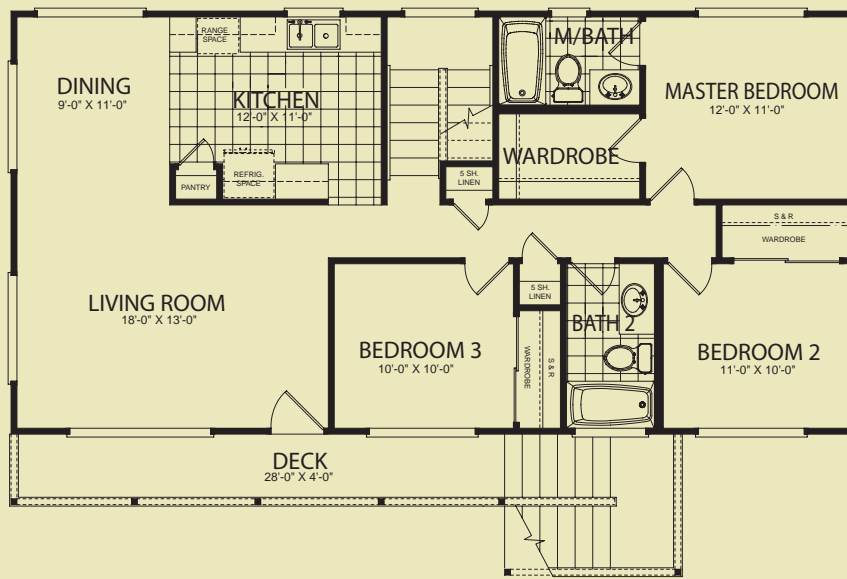
SECOND FLOOR
